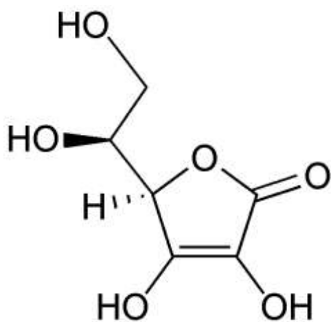
Ascorbic acid - Vitamin C
