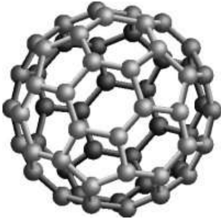
Buckminster Fullerene "Buckyball"
